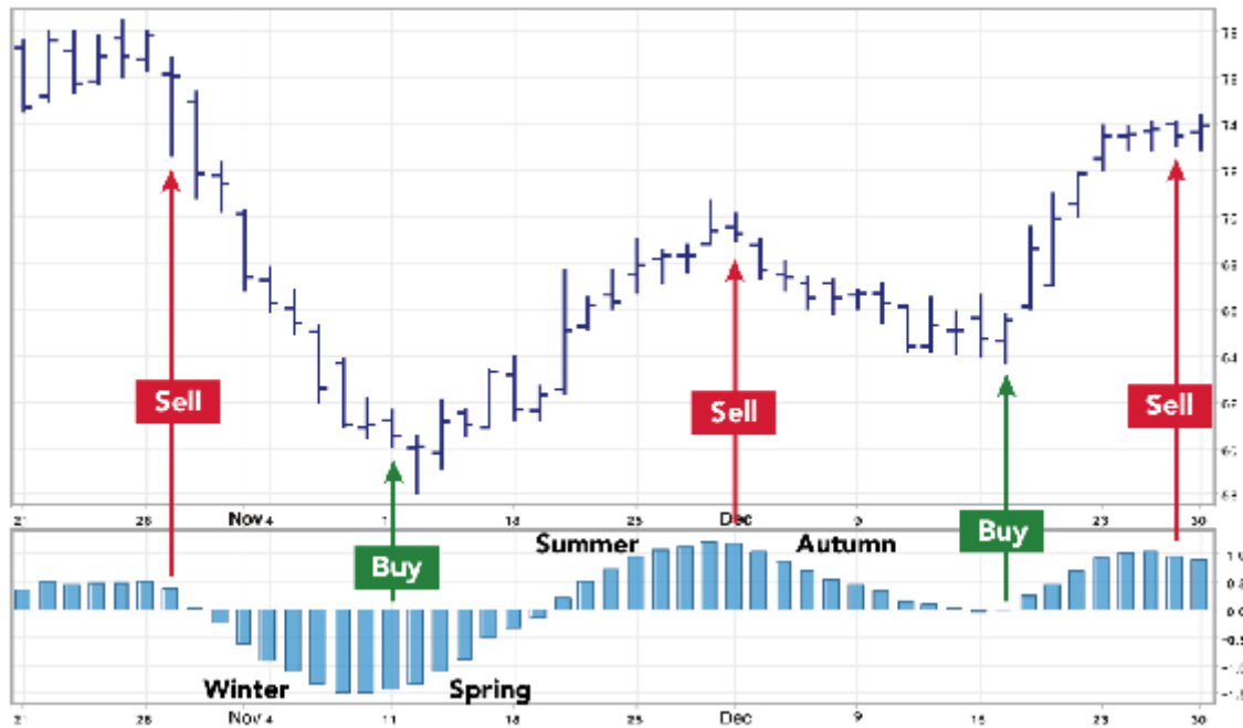
FIGURE 32.1 VRTX daily, MACD-Histogram 12-26-9. (Chart by Stockcharts.com)
